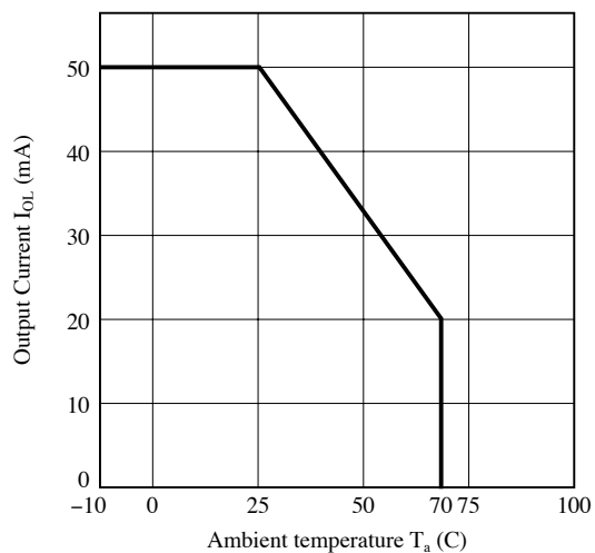
Fig.5 Output Current vs. Ambient Temperature
