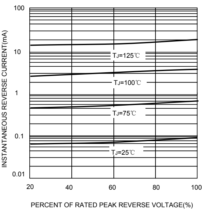
FIG.3-TYPICAL REVERSE CHARACTERISTICS
