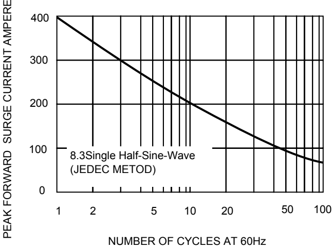
FIG.2-MAXIMUM NON-REPETITIVE SURGE
