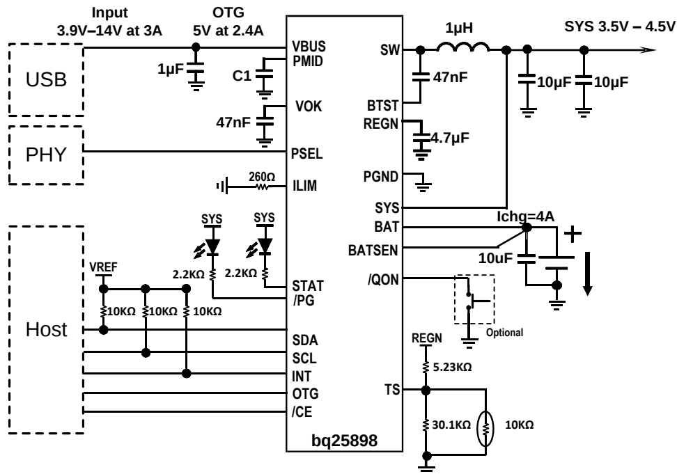
图 65. bq25898 with PSEL Interface and USB On-The-Go (OTG)
