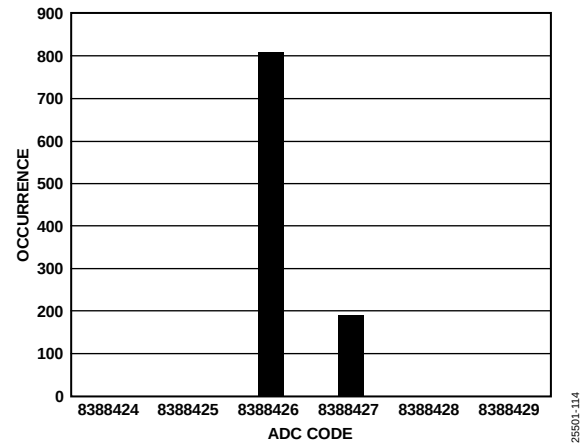
Figure 14. Histogram (Low Level Input, Output Data Rate = 1.25 SPS)
