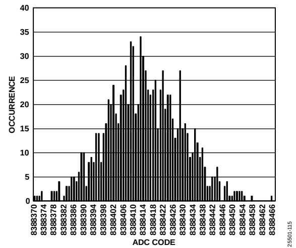
Figure 15. Histogram (Low Level Input, Output Data Rate = 5.194 kSPS)
