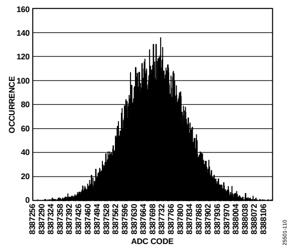
Figure 10. Histogram (Voltage Input, Output Data Rate = 62.5 kSPS)
