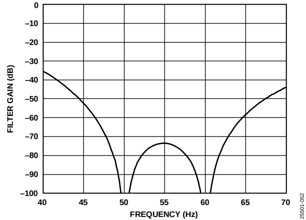
Figure 54. 20 SPS ODR, 50 ms Settling Time (40 Hz to 70 Hz)
