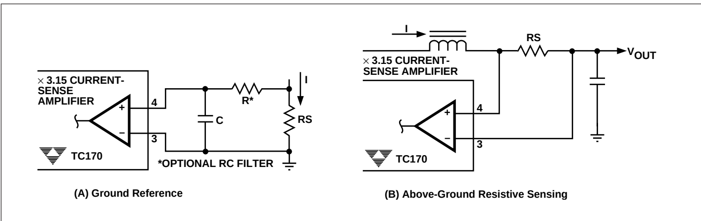
Figure 2. Resistive Sensing
