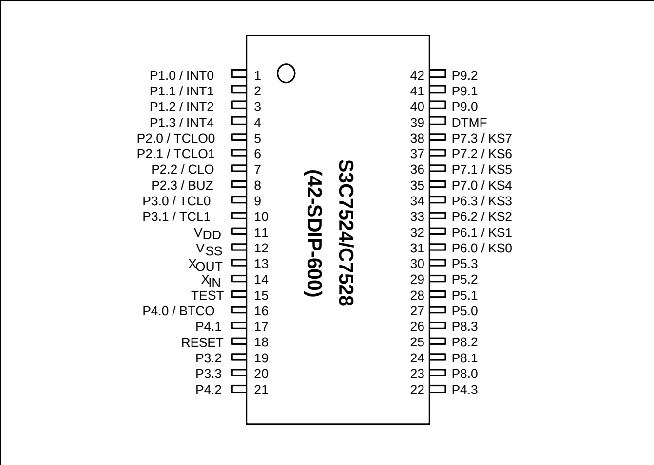
Figure 1-2. S3C7524/C7528 Pin Assignment Diagrams (42-SDIP)
