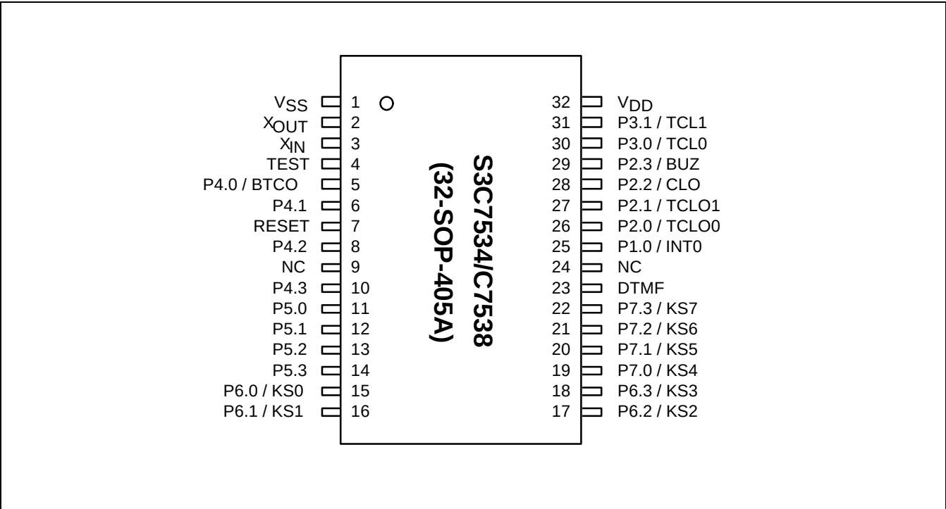
Figure 1-5. S3C7534/C7538 Pin Assignment Diagrams (32-SOP)
