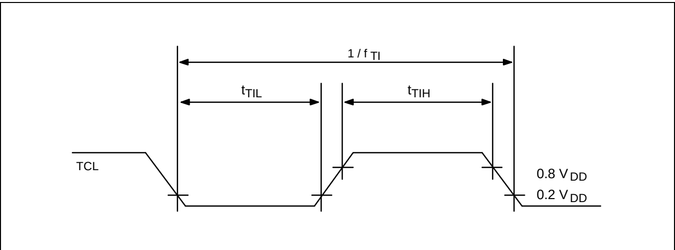
Figure 13-6. TCL Timing
