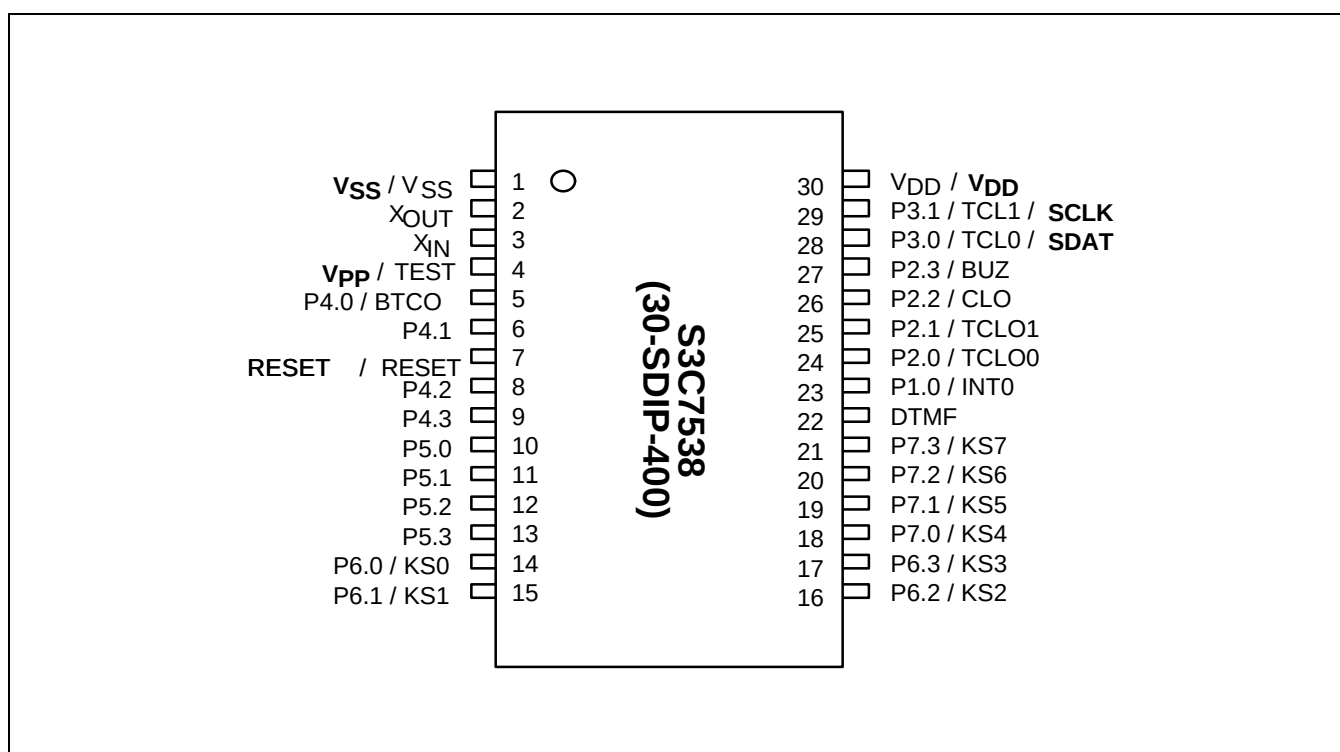
Figure 15-3. S3P7538 Pin Assignments (30-SDIP)
