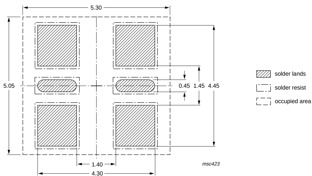
Fig 20. Reflow soldering footprint
