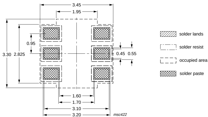
Fig 20. Reflow soldering footprint
