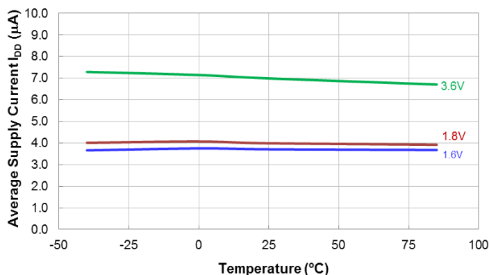
Average Supply Current vs Temperature
