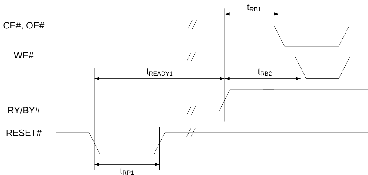
Figure 14. AC Waveforms for RESET# Reset# Timings
