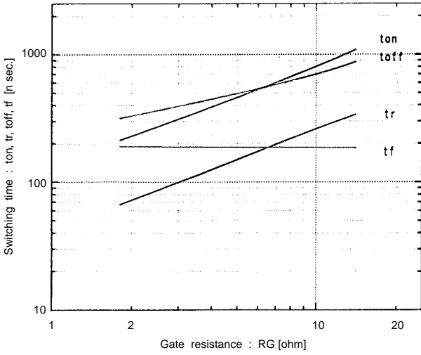
Switching time vs. RG Vcc=300V, Ic=300A, VGE=±15V, Tj=25°C
