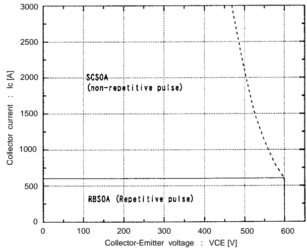
Reversed biased safe operating area +VGE=15V, -VGE ≤ 15V, Tj ≤ 125°C, RG ≥ 6.8 ohm
