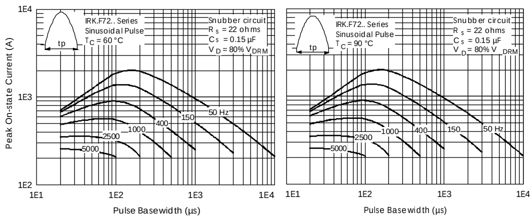
Fig. 11 - Frequency Characteristics
