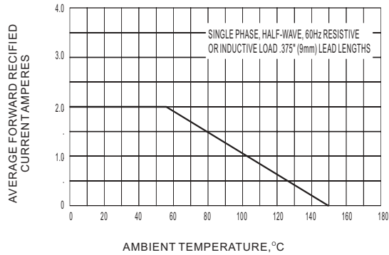
FIG.1 MAXIMUM AVERAGE FORWARD CURRENT RATING
