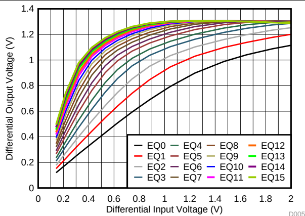
Figure 3. USB RX EQ Settings Curves
