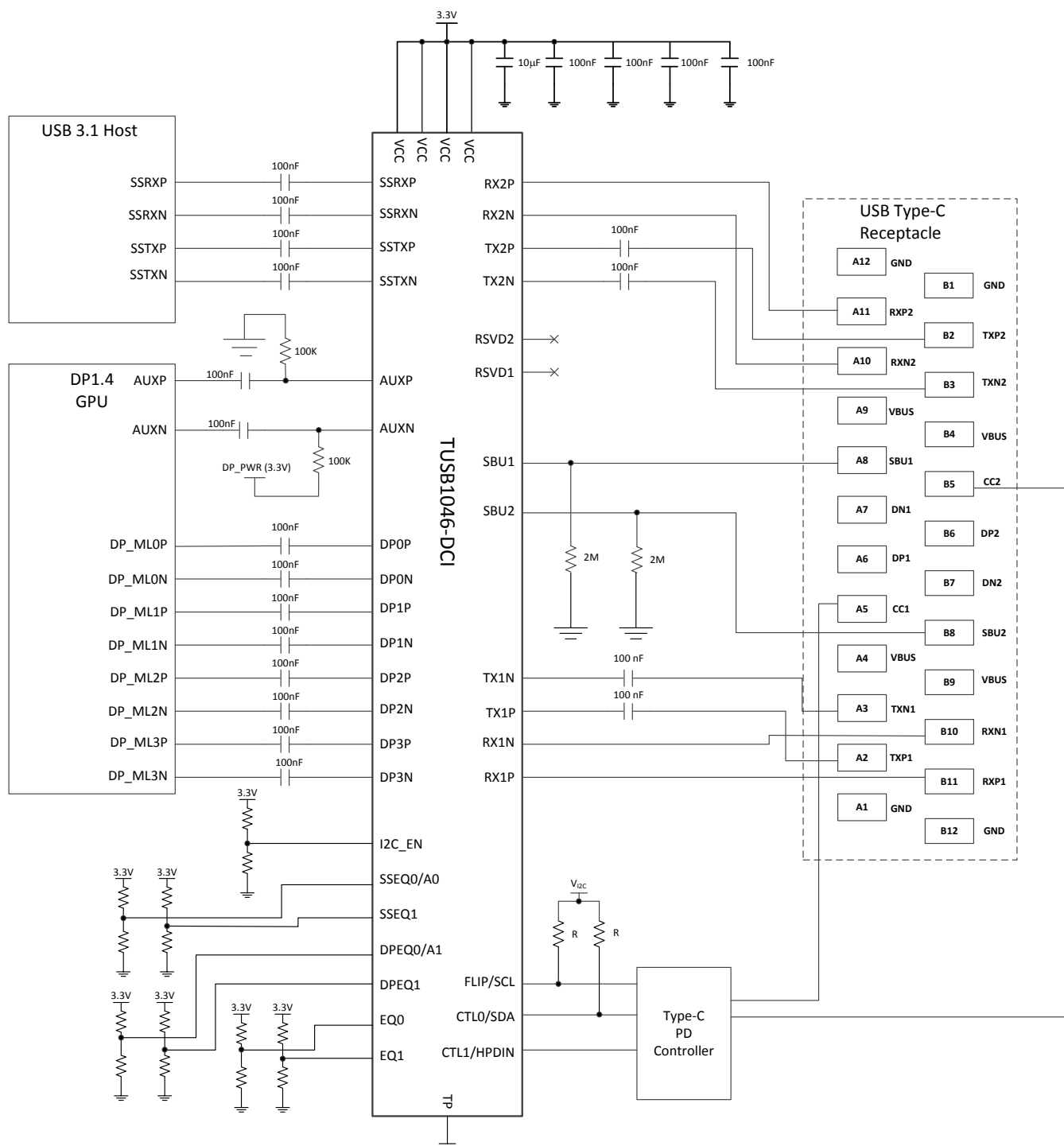
Figure 27. Application Circuit
