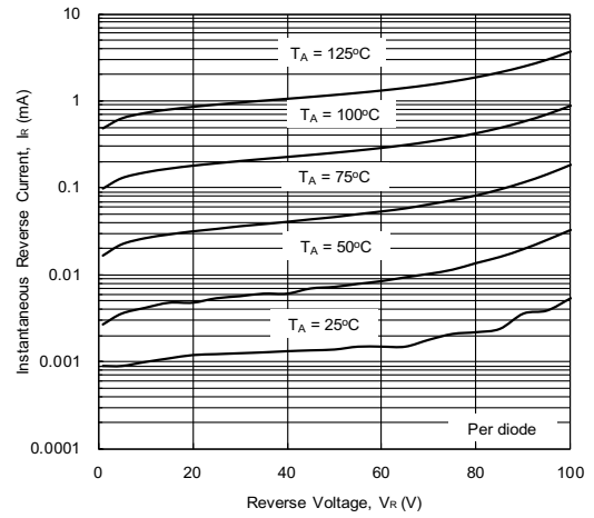
Fig. 2 - Reverse Characteristics
