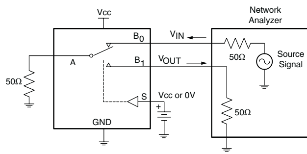
Figure 4. Crosstalk
