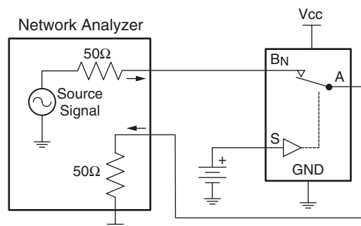
Figure 7. Bandwidth
