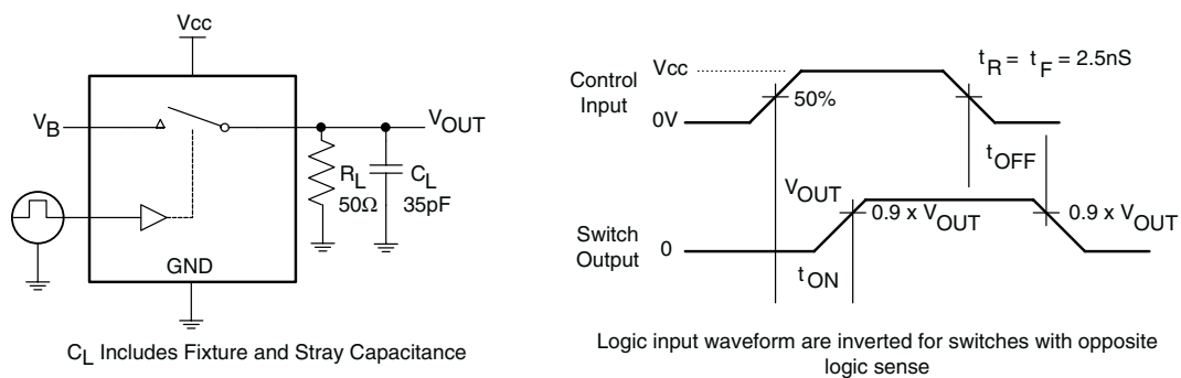
Figure 1. Turn-On/Turn-Off Timing
