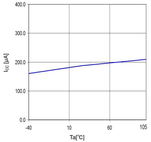
Figure 22. T_a - I_{cc}
