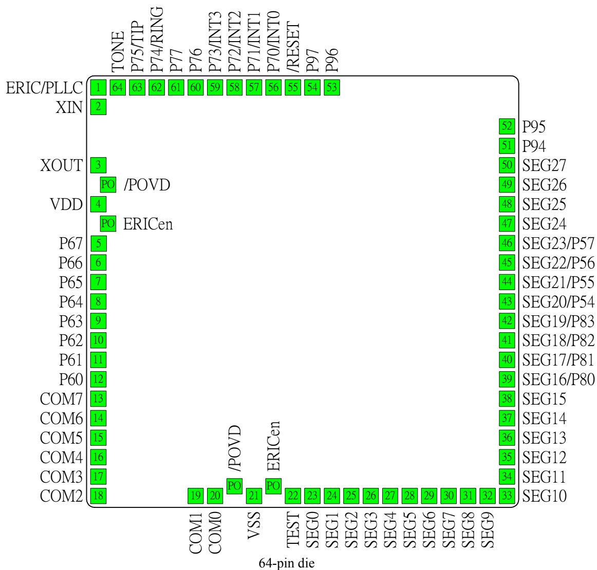
Fig.1 Pad assignment
