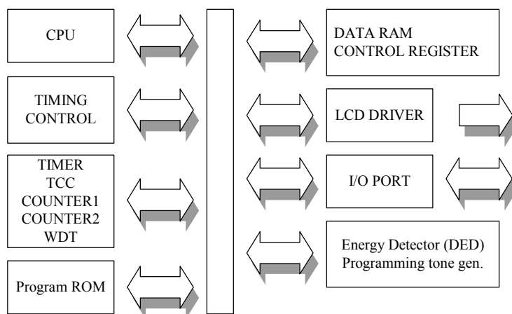
Fig.2 Block diagram1
