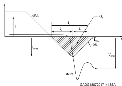
Figure 21: Diode reverse recovery waveform
