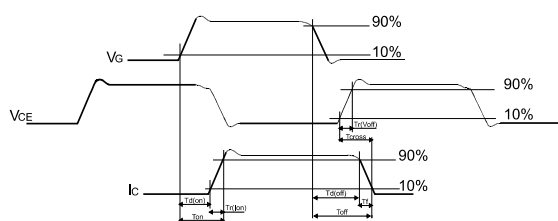
Figure 20: Switching waveform
