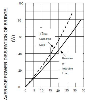
FIG.6-MAXIMUM POWER DISSIPATION
