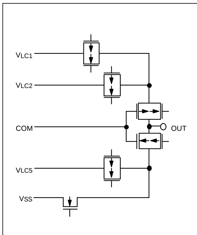
Figure 1-9. Pin Circuit Type H-4
