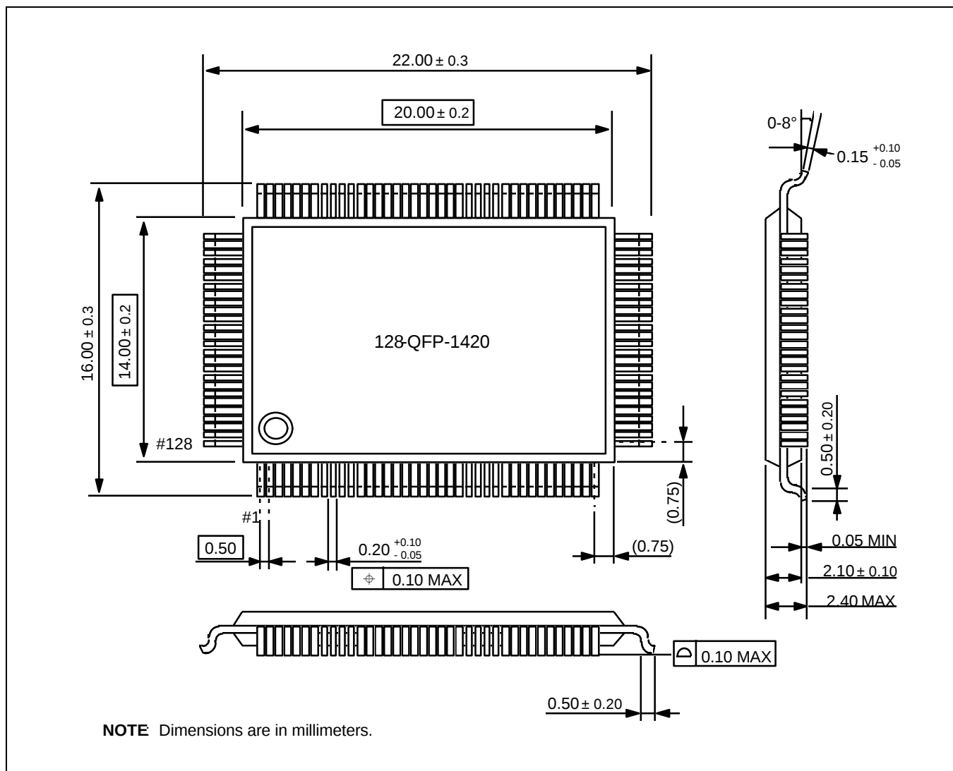
Figure 16-1. 128-QFP-1420 Package Dimensions
