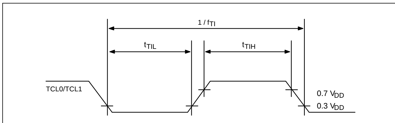
Figure 15-7. TCL0/TCL1 Timing
