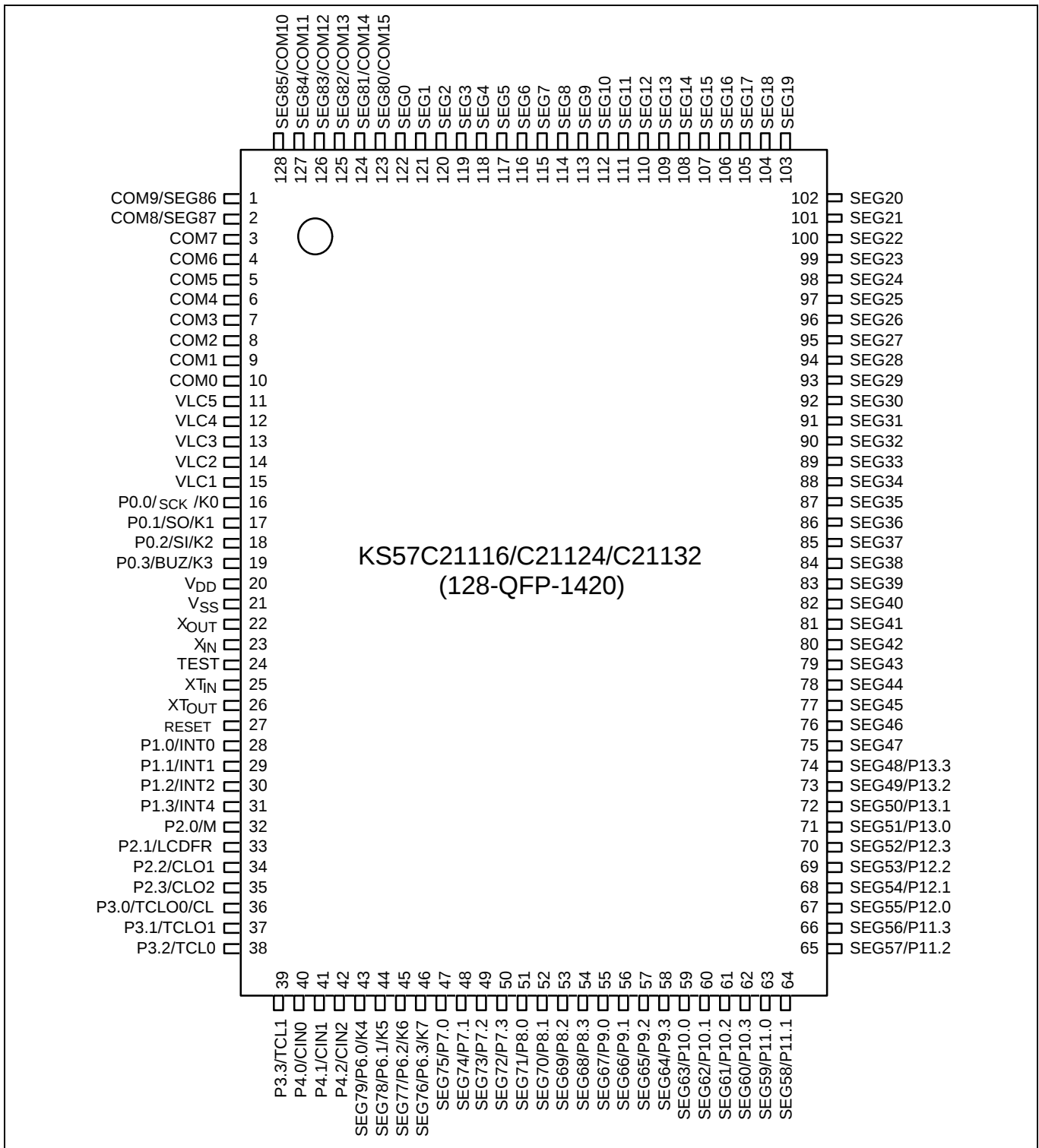
Figure 1-2. KS57C21116/C21124/C21132 128-QFP Pin Assignment
