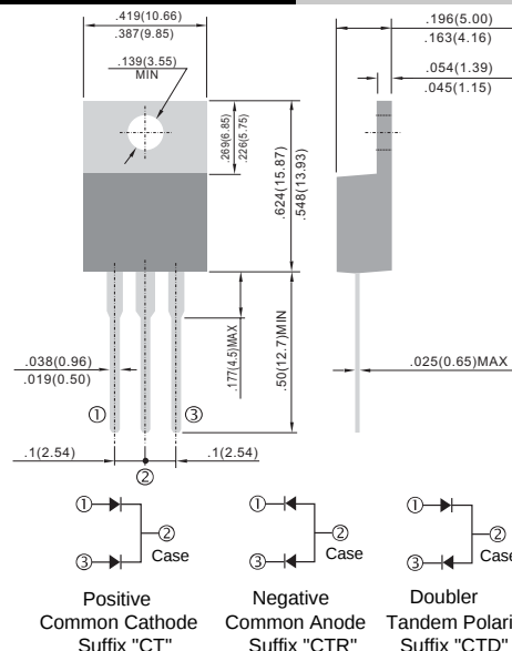
TO-220AB
