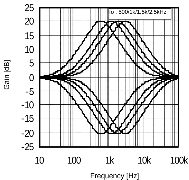
Figure 8. Middle fo vs Frequency
