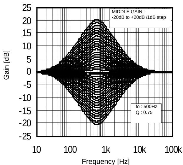
Figure 7. Middle Gain vs Frequency
