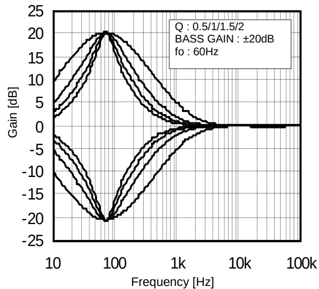
Figure 6. Bass Q vs Frequency
