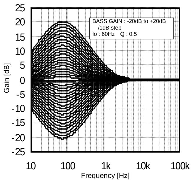
Figure 4. Bass Gain vs Frequency
