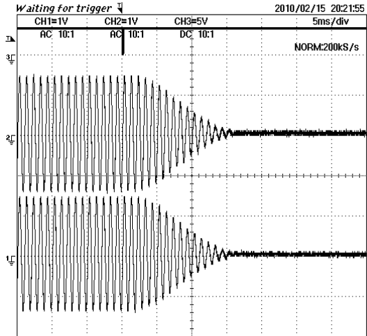
Figure 20. Advanced Switch 2
