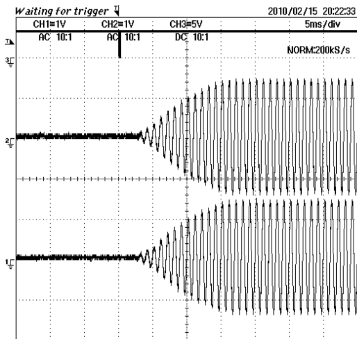
Figure 19. Advanced Switch 1
