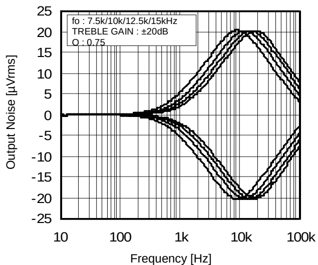
Figure 11. Treble fo vs Frequency
