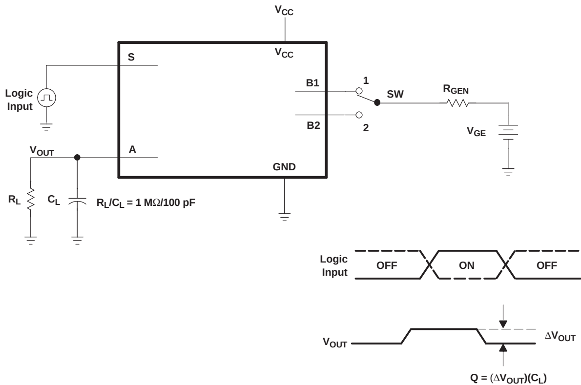
Figure 9. Charge-Injection Test
