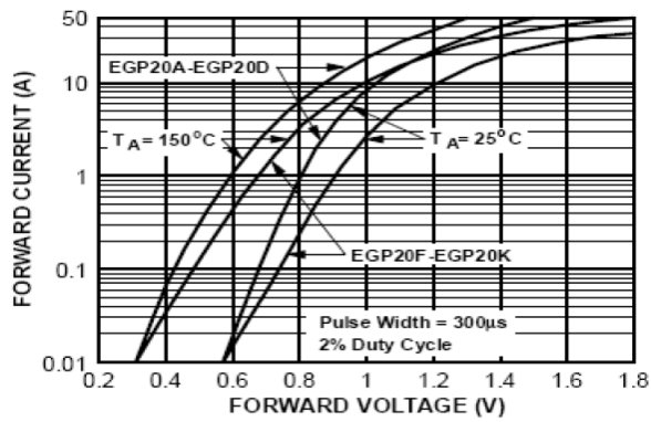
Figure 3. Forward Characteristics
