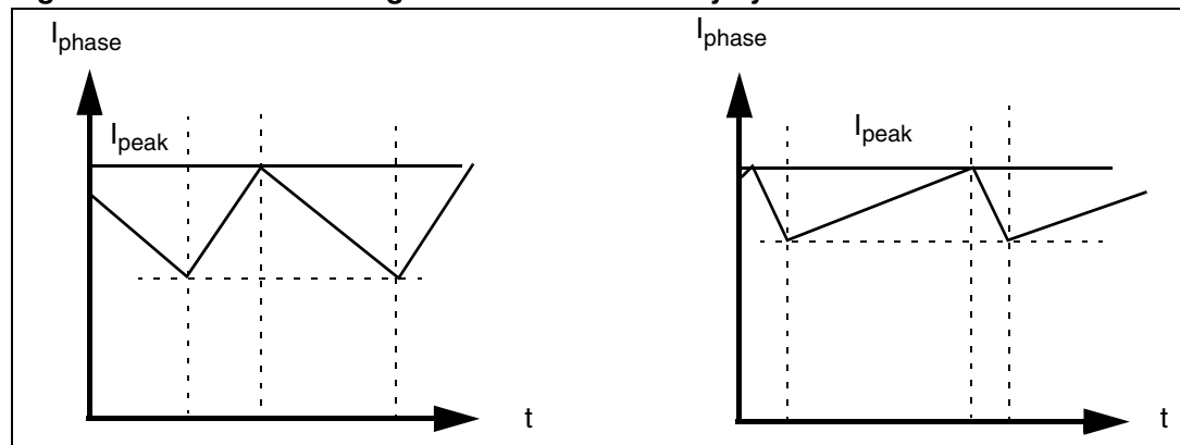
Figure 1. Peak current regulation at different duty cycles with BEMF load
