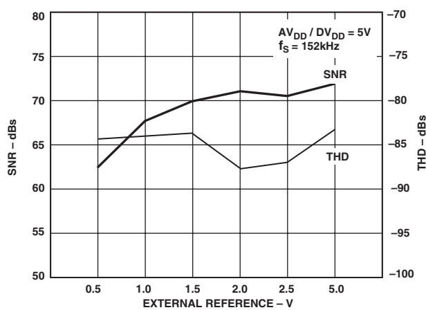
TPC 13. Typical Dynamic Performance vs. V_{REF} , V_{DD} = 5\text{ V}
