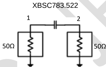
Schematic of 22nF XBSC in transmission mode
