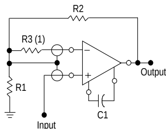
Noninverting Amplifier
