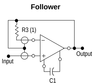
Figure 9. Connection of Input Guards
