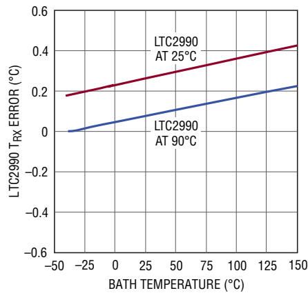
Remote Diode Error with LTC2990 at 25^\circ\text{C} , 90^\circ\text{C}
