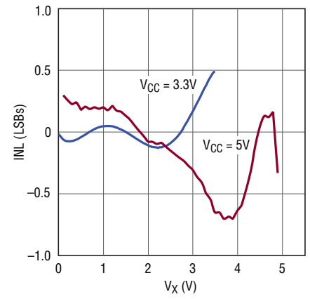
Single-Ended INL
