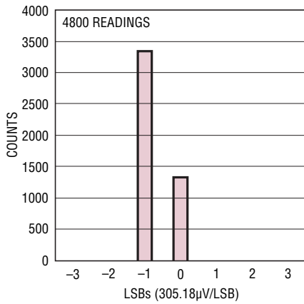
Single-Ended Noise
