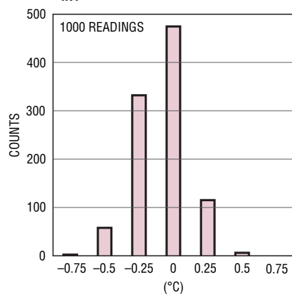
T INT Noise
