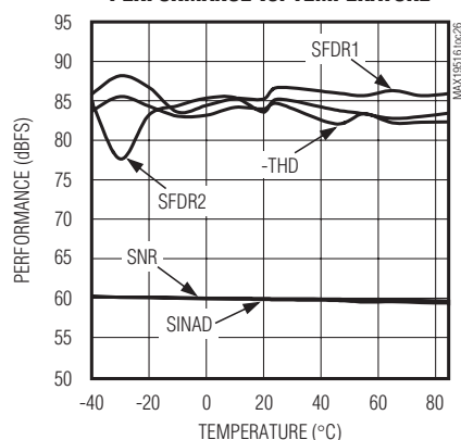
PERFORMANCE vs. TEMPERATURE
