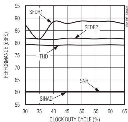
PERFORMANCE vs. CLOCK DUTY CYCLE
