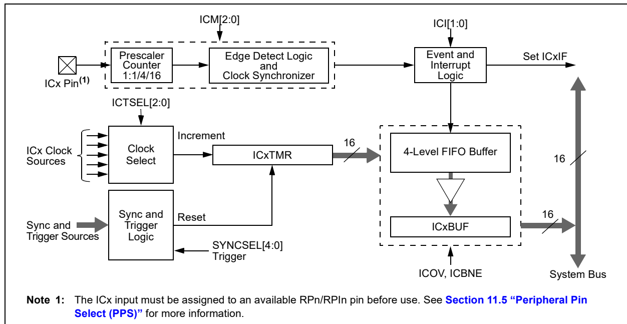
FIGURE 14-1: INPUT CAPTURE x BLOCK DIAGRAM
