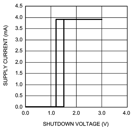
Shutdown Hysteresis Voltage V_{DD} = 5V , SD Mode = V_{DD} (Low)
