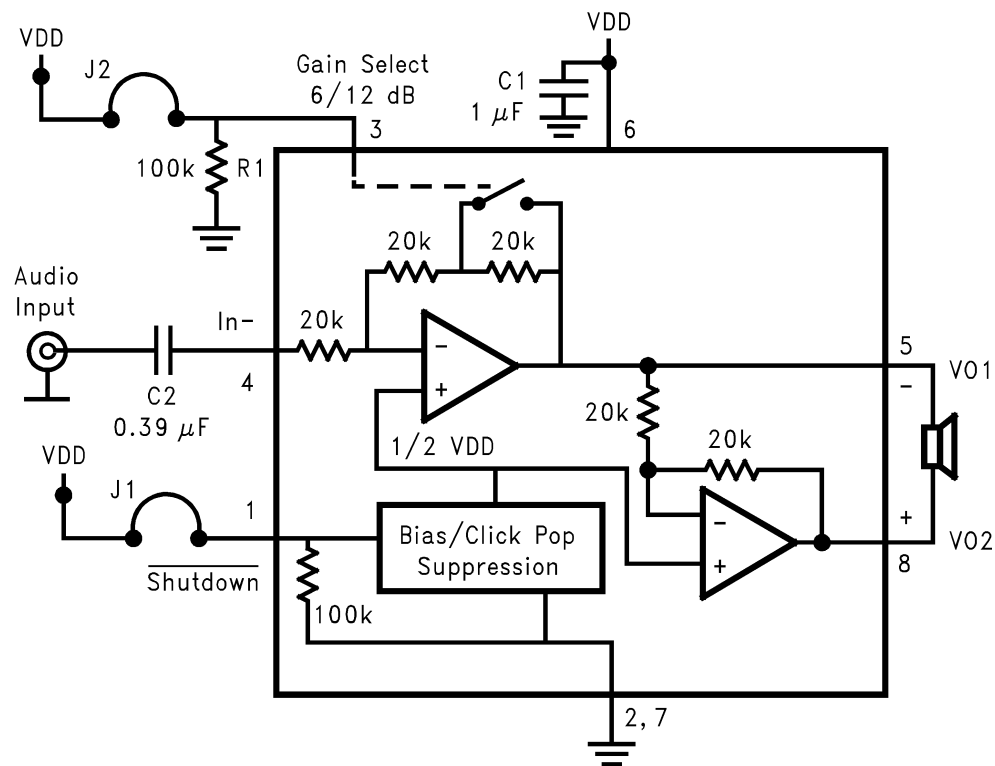
FIGURE 2. REFERENCE DESIGN BOARD SCHEMATIC
