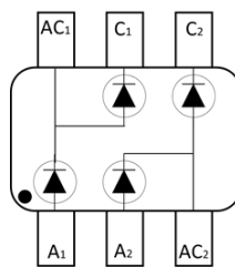
BAS40BDW
