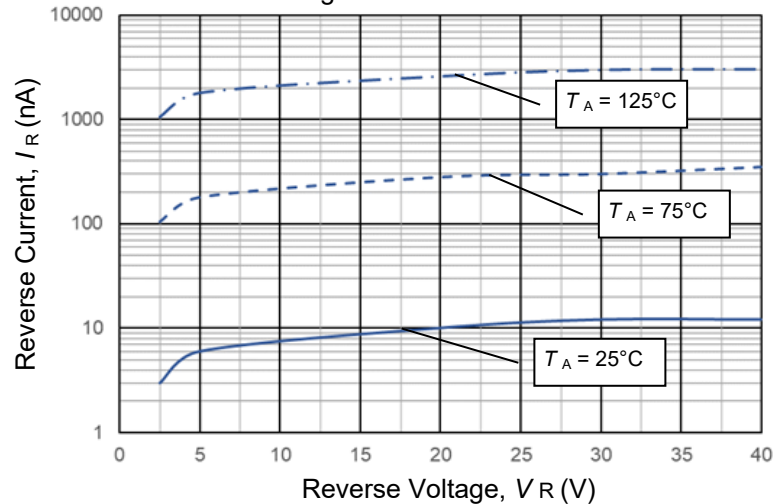
Fig 2. Reverse Current
