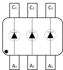
BAS40DW
