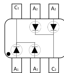
BAS40CDW
