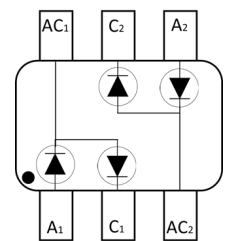
BAS40SDW
