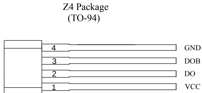
Figure 2. Pin Configuration of AH9279 (Front View)
