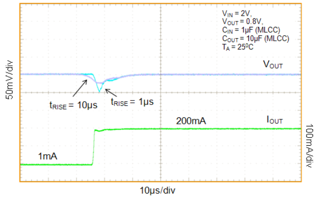
Figure 53. Load Transient Response – Rising Edge, I_{OUT} = 1mA - 200mA , C_{OUT} = 10\mu F
