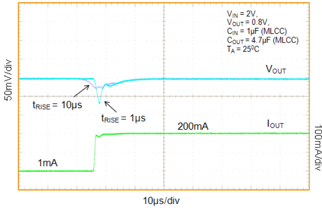
Figure 51. Load Transient Response – Rising Edge, I_{OUT} = 1mA - 200mA , C_{OUT} = 4.7\mu F
