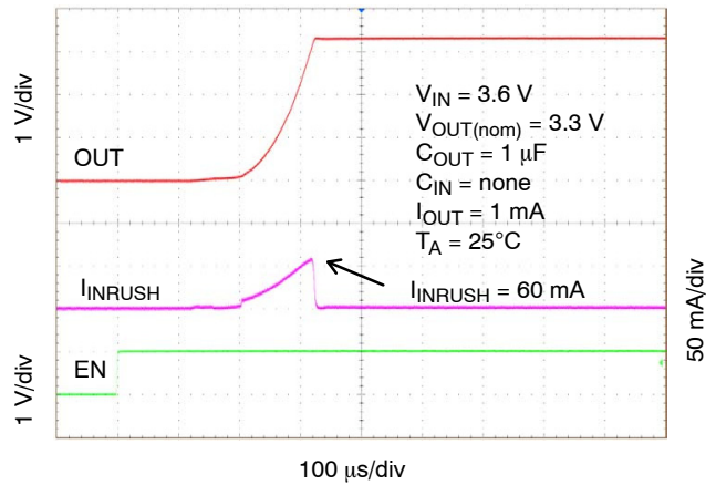
Figure 36. Enable Turn-On Response, V_{OUT} = 3.3\text{ V} , C_{OUT} = 1\text{ μF}
