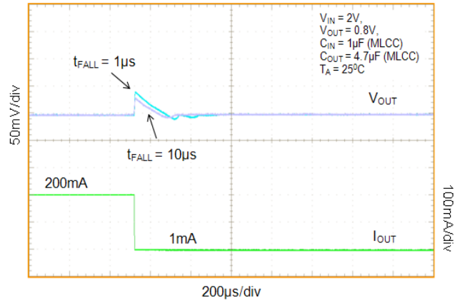
Figure 52. Load Transient Response – Falling Edge, I_{OUT} = 1mA - 200mA , C_{OUT} = 4.7\mu F
