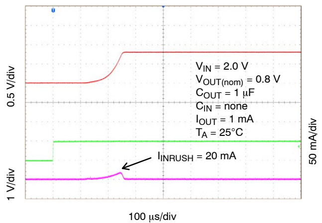
Figure 38. Enable Turn-On Response, V_{OUT} = 0.8\text{ V} , C_{OUT} = 1\text{ μF}
