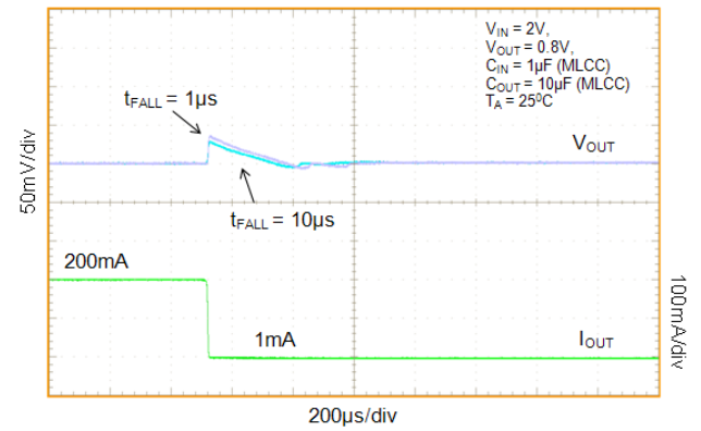
Figure 54. Load Transient Response – Falling Edge, I_{OUT} = 1mA - 200mA , C_{OUT} = 10\mu F
