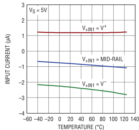
Input Bias Current vs Temperature, Op Amp 1
