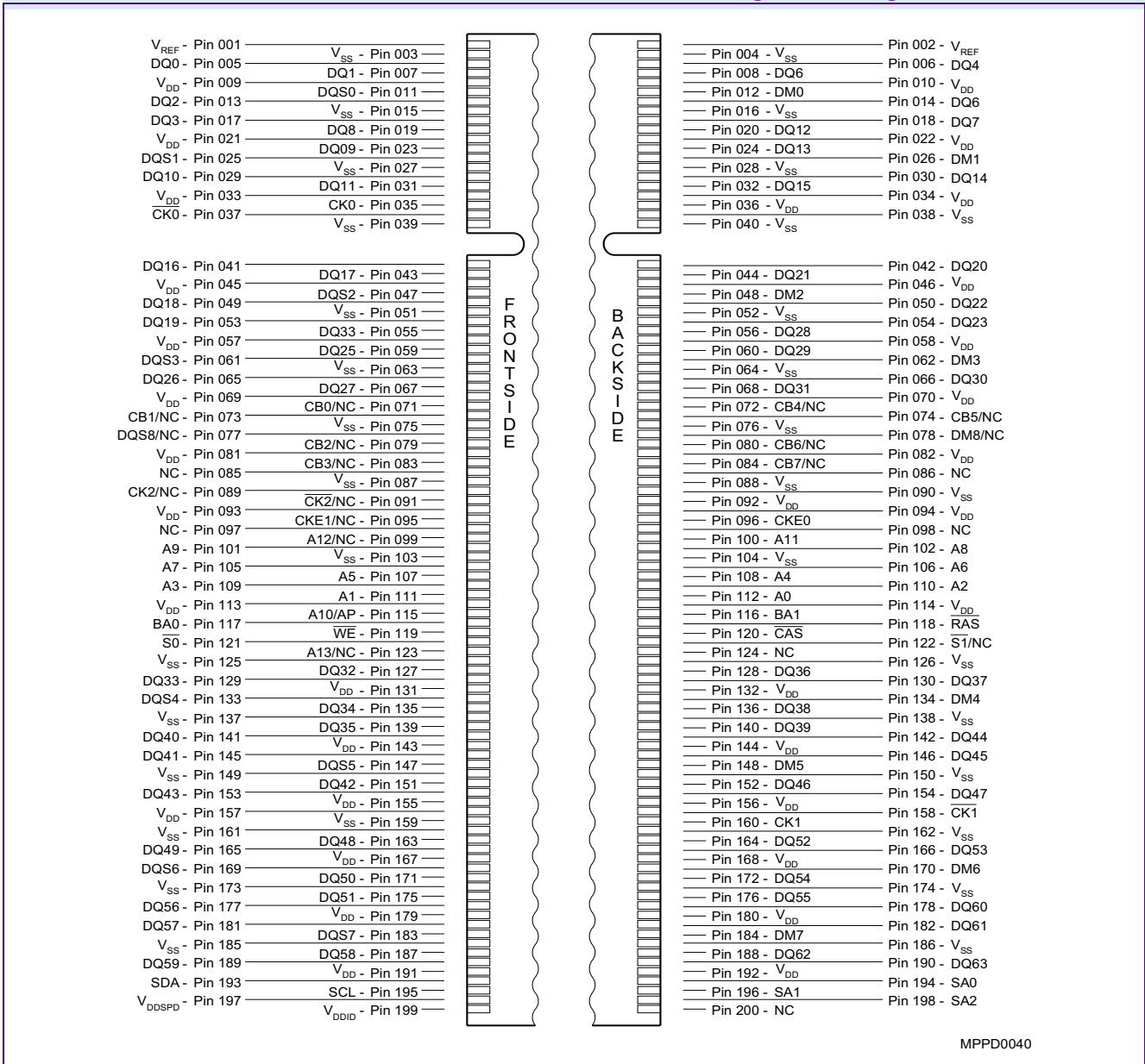
FIGURE 1 Pin Configuration Diagram 200-Pin SO-DIMM
