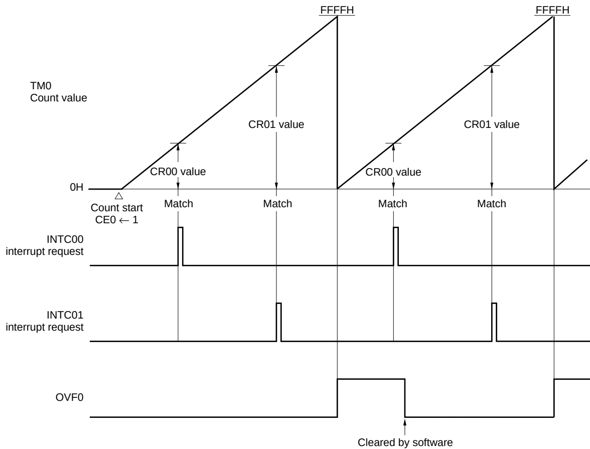
Figure 9-13. Compare Operation
