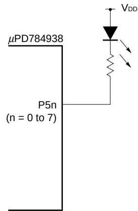
Figure 6-50. Example of Direct LED Drive
