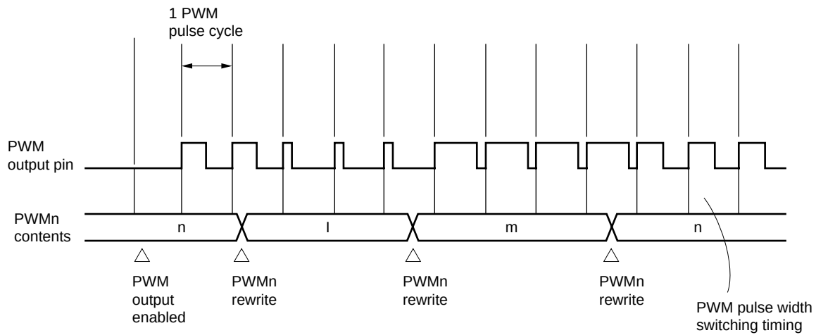
Figure 15-7. PWM Output Timing Example 2 (PWM pulse width rewrite cycle = 2^8/f_{\text{PWM}} )
