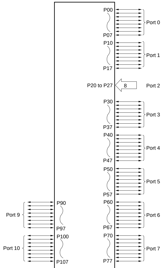
Figure 6-1. Port Configuration
