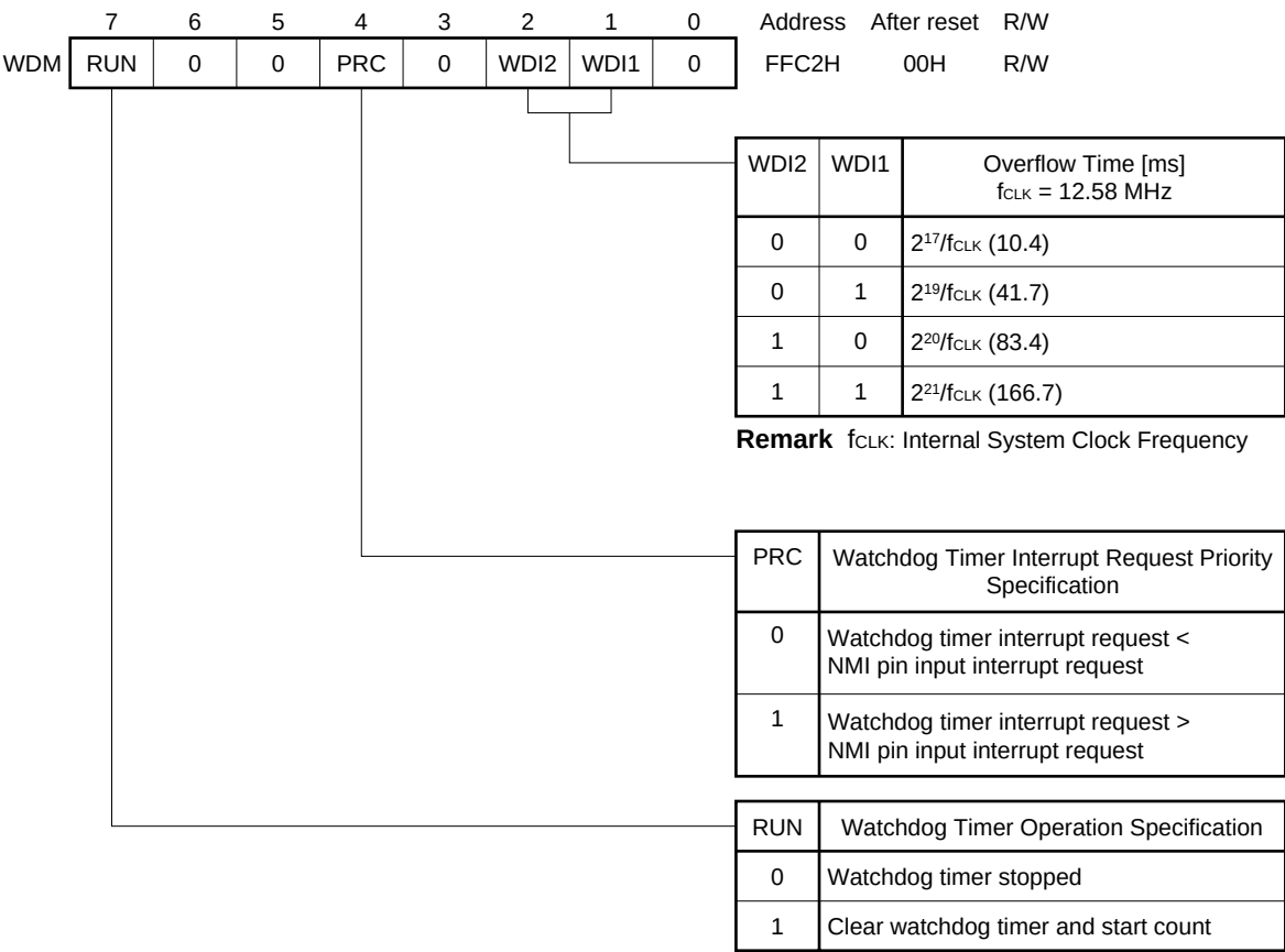
Figure 13-2. Watchdog Timer Mode Register (WDM) Format
