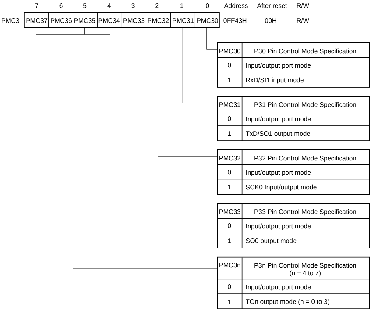
Figure 6-31. Port 3 Mode Control Register (PMC3) Format
