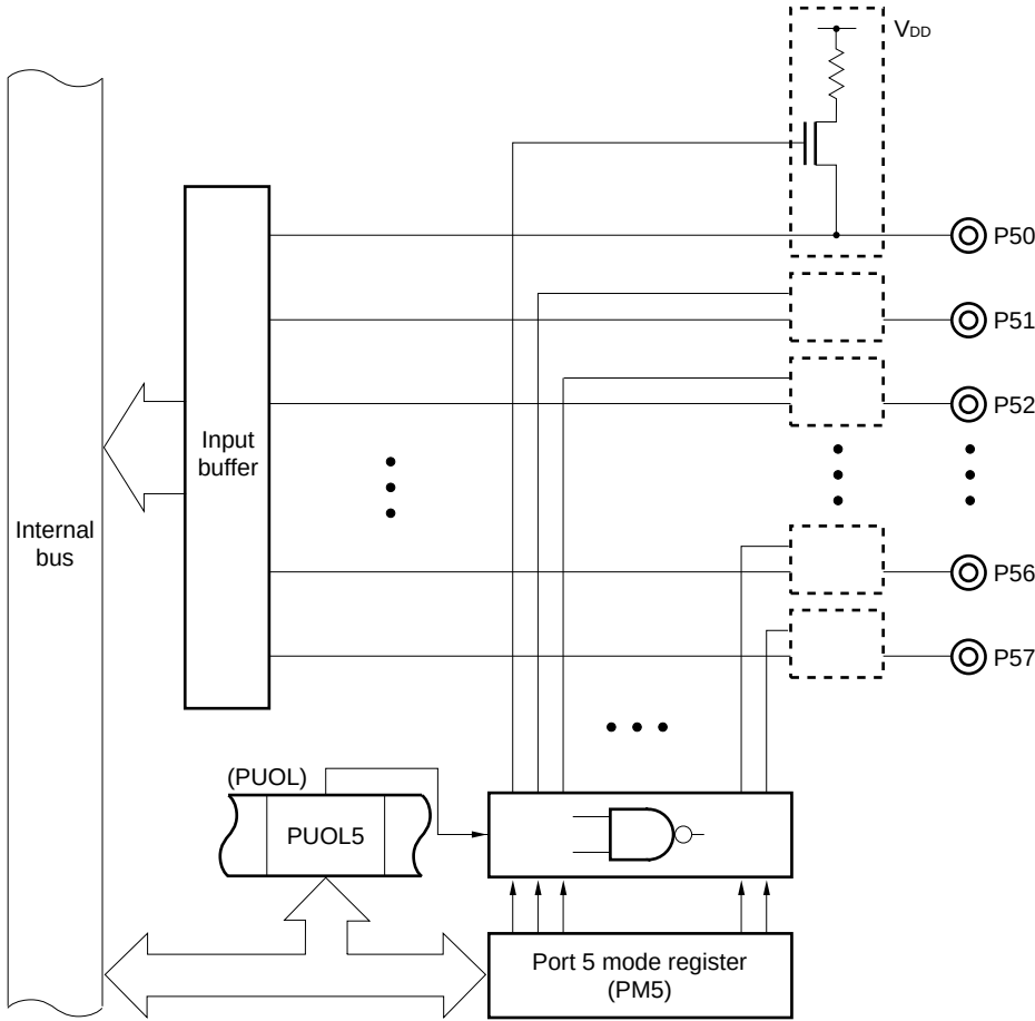
Figure 6-49. Pull-Up Specification (Port 5)
