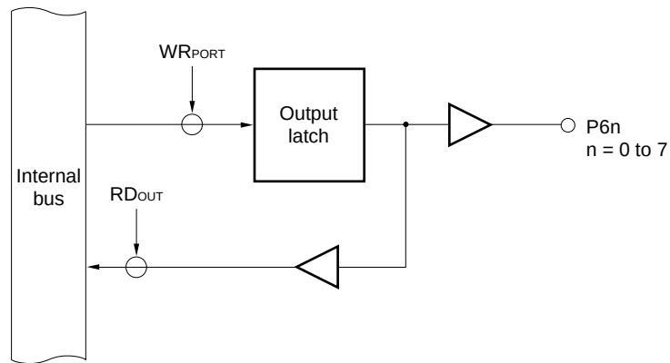
Figure 6-56. Port Specified as Output Port
