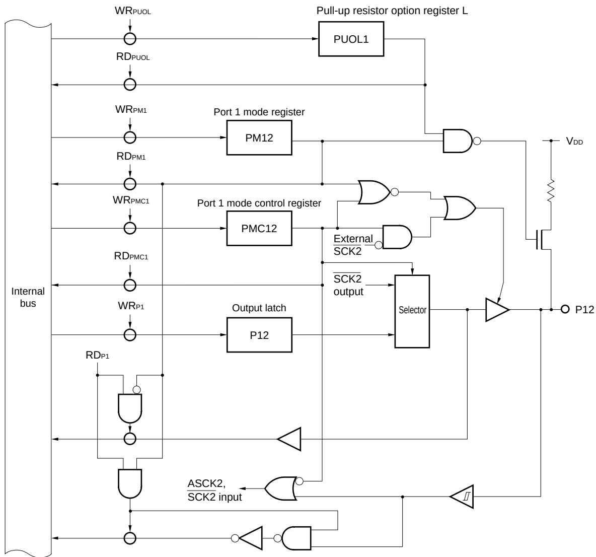
Figure 6-9. P12 (Port 1) Block Diagram
