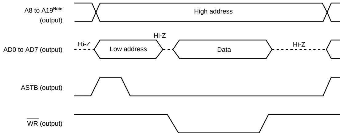
Figure 24-7. Write Timing
