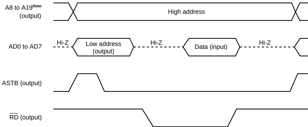
Figure 24-6. Read Timing
