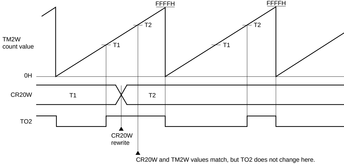
Figure 11-26. Example of Compare Register (CR20W) Rewrite
