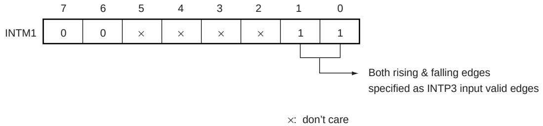
Figure 9-39. Pulse Width Measurement Setting Procedure
