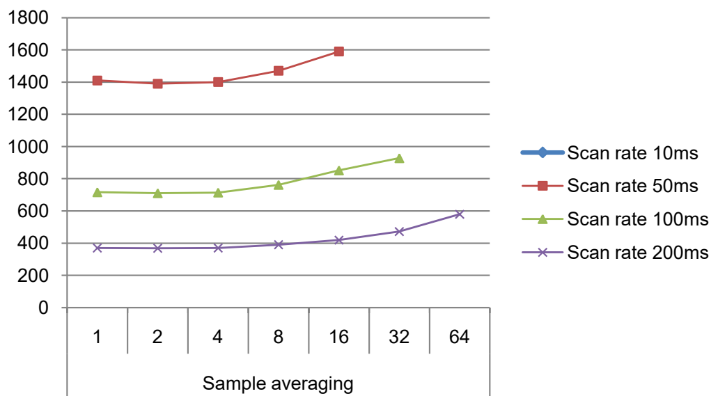
Figure 41-12. Power Consumption [ \mu A] 100 sensors, noise countermeasures Enabled, f=48\text{MHz} , V_{CC}=3.3\text{V}
