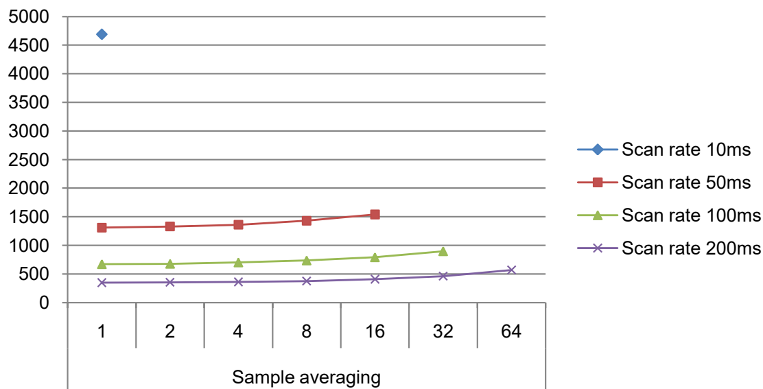
Figure 41-12. Power Consumption [ \mu A] 100 sensors, noise countermeasures Enabled, f=48\text{MHz} , V_{CC}=3.3\text{V}
