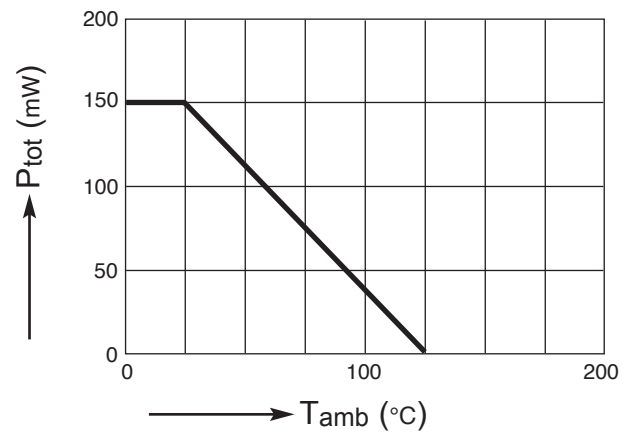
FIG. 5 - ADMISSIBLE POWER DISSIPATION VERSUS AMBIENT TEMPERATURE
