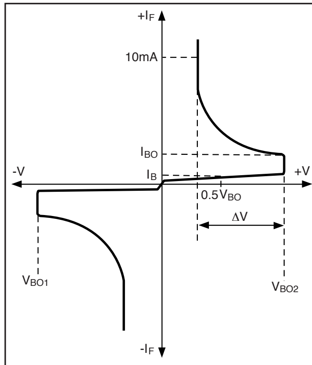
FIG. 1 - CURRENT-VOLTAGE CHARACTERISTICS
