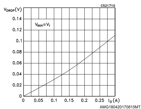
Figure 16: Dropout voltage vs output current
