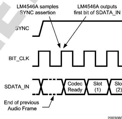
FIGURE 7. Start of AC Link Input Frame
