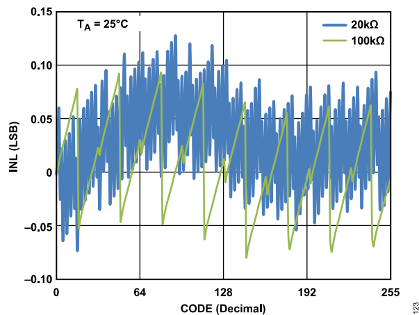
Figure 16. R-INL in R-Perf Mode vs. Code vs. Nominal Resistance (AD5271)
