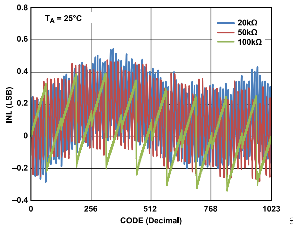
Figure 8. R-INL in R-Perf Mode vs. Code vs. Nominal Resistance (AD5270)
