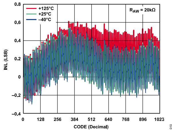
Figure 7. R-INL in R-Perf Mode vs. Code vs. Temperature (AD5270)
