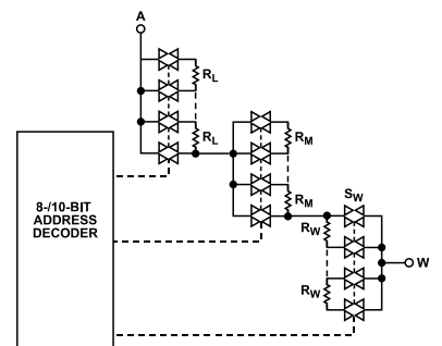
Figure 45. Simplified RDAC Circuit
