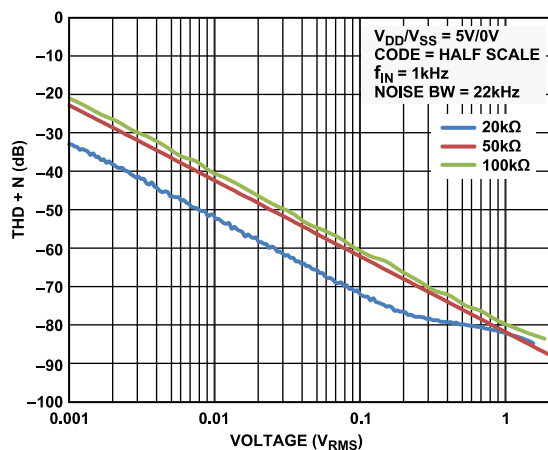
Figure 32. THD + N vs. Amplitude
