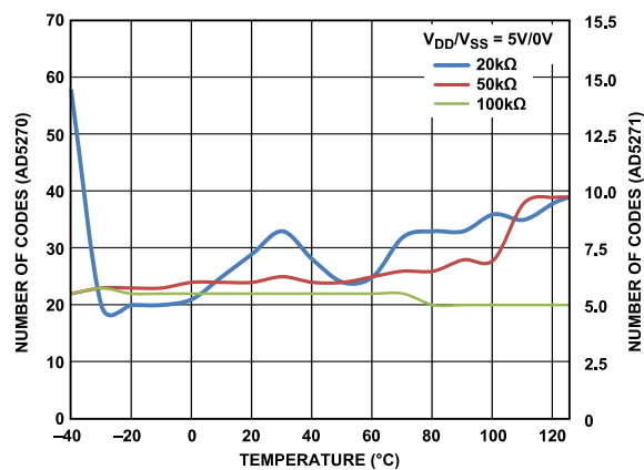
Figure 35. Maximum Code Loss &gt; 1% R-Tolerance Error vs. Temperature
