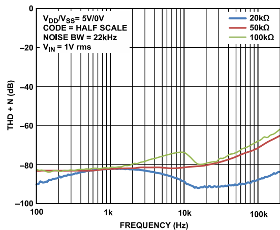
Figure 31. THD + N vs. Frequency
