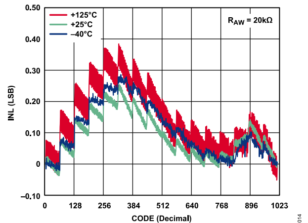
Figure 11. R-INL in Normal Mode vs. Code vs. Temperature (AD5270)
