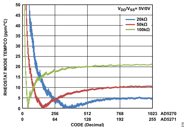
Figure 25. Tempco \Delta R_{WA}/\Delta T vs. Code
