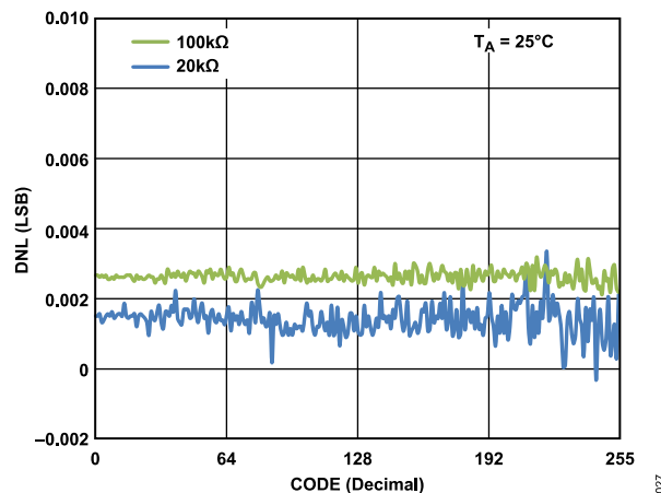
Figure 22. R-DNL in Normal Mode vs. Code vs. Nominal Resistance (AD5271)
