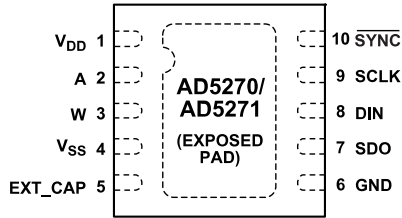
Figure 6. LFCSP Pin Configuration
