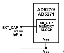
Figure 46. EXT_CAP Hardware Setup
