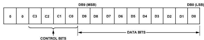
Figure 2. Shift Register Content
