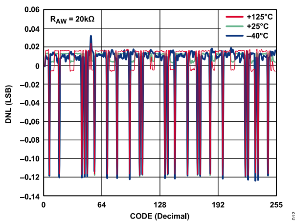
Figure 17. R-DNL in R-Perf Mode vs. Code vs. Temperature (AD5271)
