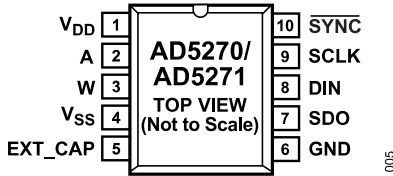
Figure 5. MSOP Pin Configuration
