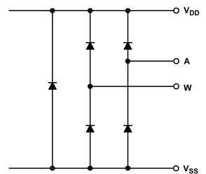
Figure 47. Maximum Terminal Voltages Set by V_{DD} and V_{SS}
