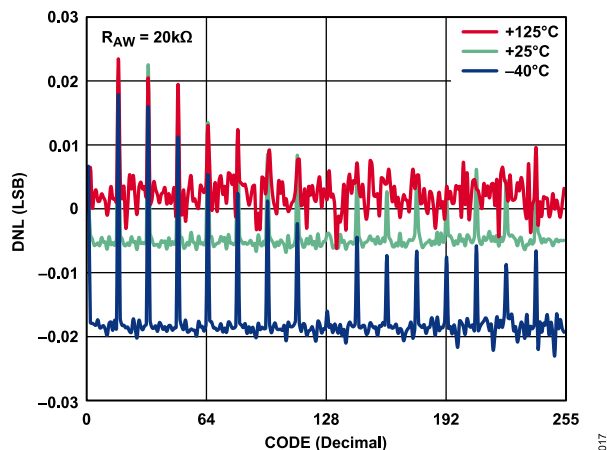
Figure 21. R-DNL in Normal Mode vs. Code vs. Temperature (AD5271)
