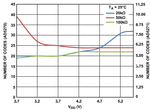
Figure 34. Maximum Code Loss &gt; 1% R-Tolerance Error vs. Voltage
