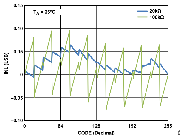
Figure 20. R-INL in Normal Mode vs. Code vs. Nominal Resistance (AD5271)
