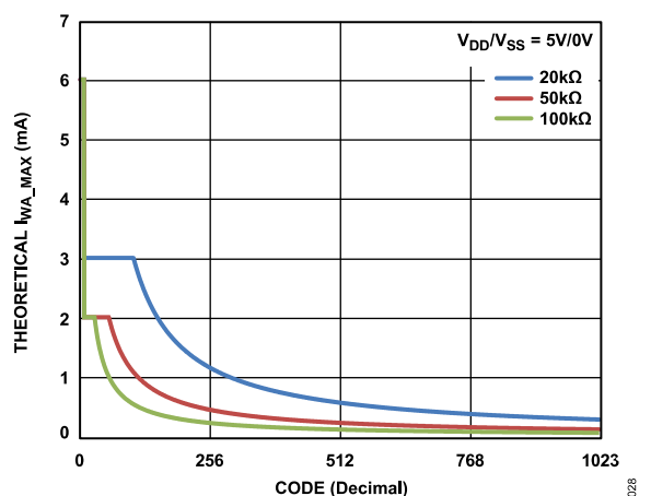
Figure 26. Theoretical Maximum Current vs. Code
