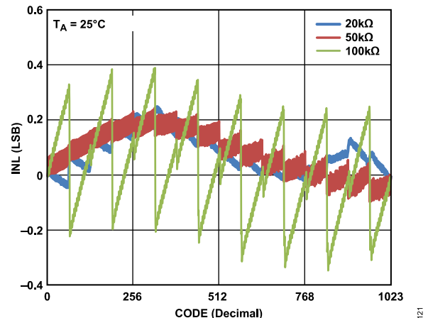
Figure 12. R-INL in Normal Mode vs. Code vs. Nominal Resistance (AD5270)
