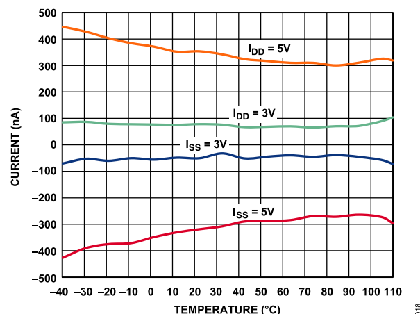
Figure 23. Supply Current ( I_{DD} , I_{SS} ) vs. Temperature
