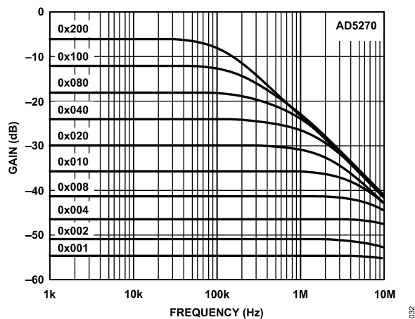
Figure 28. 50 kΩ Gain vs. Code vs. Frequency
