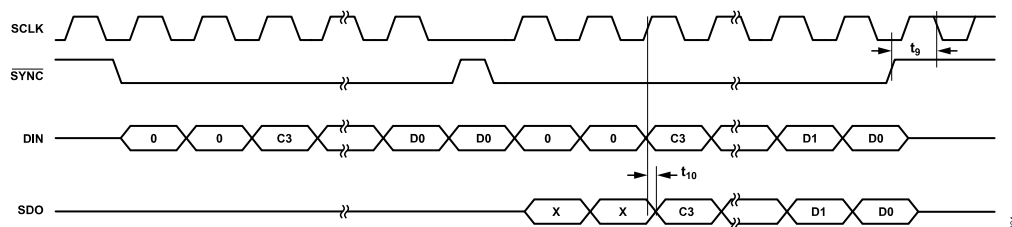
Figure 4. Read Timing Diagram (CPOL = 0, CPHA = 1)
