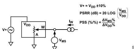
Figure 41. Power Supply Sensitivity (PSS, PSRR)
