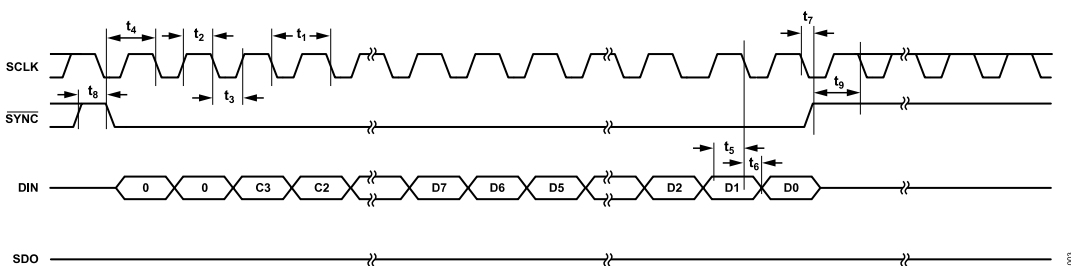
Figure 3. Write Timing Diagram (CPOL = 0, CPHA = 1)
