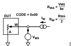
Figure 40. Wiper Resistance
