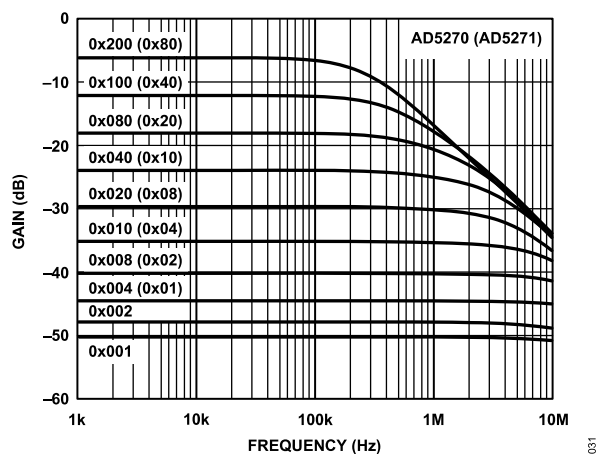
Figure 27. 20 kΩ Gain vs. Code vs. Frequency
