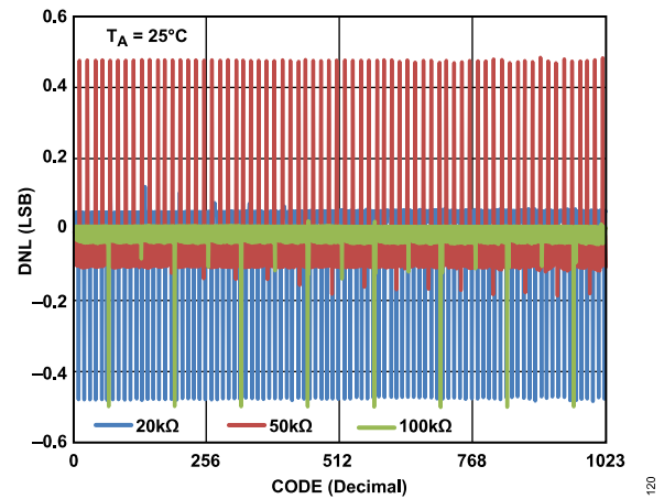
Figure 10. R-DNL in R-Perf Mode vs. Code vs. Nominal Resistance (AD5270)
