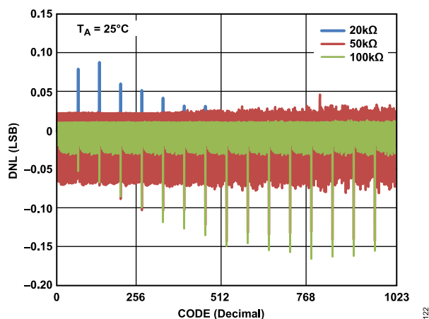
Figure 14. R-DNL in Normal Mode vs. Code vs. Nominal Resistance (AD5270)
