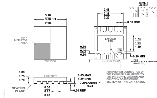
Figure 49. 10-Lead Frame Chip Scale Package [LFCSP] 3 mm x 3 mm Body and 0.75 mm Package Height (CP-10-9) Dimensions shown in millimeters
