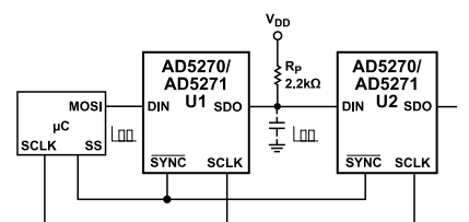
Figure 44. Daisy-Chain Configuration Using SDO
