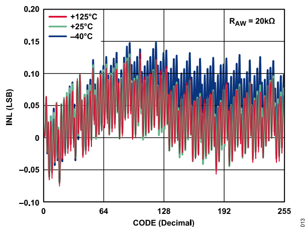
Figure 15. R-INL in R-Perf Mode vs. Code vs. Temperature (AD5271)
