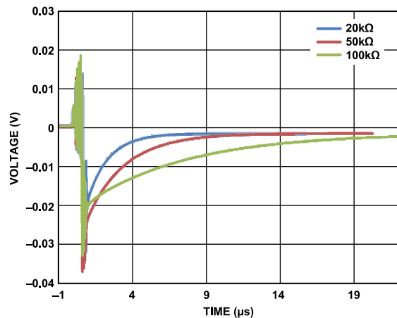
Figure 33. Maximum Glitch Energy
