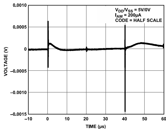
Figure 36. Digital Feedthrough
