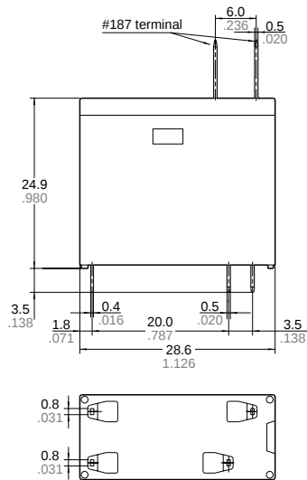
External dimensions
