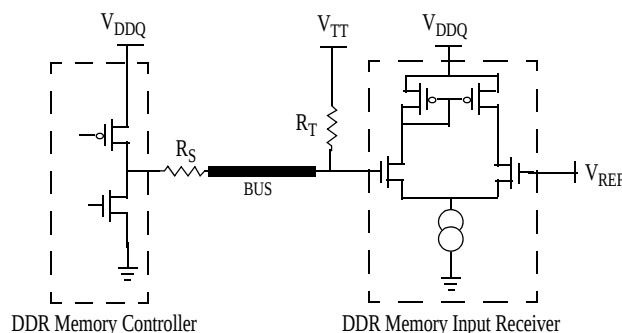
Figure 4. DDR System Level Diagram
