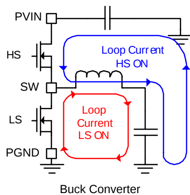
Figure 10. Current Loops
