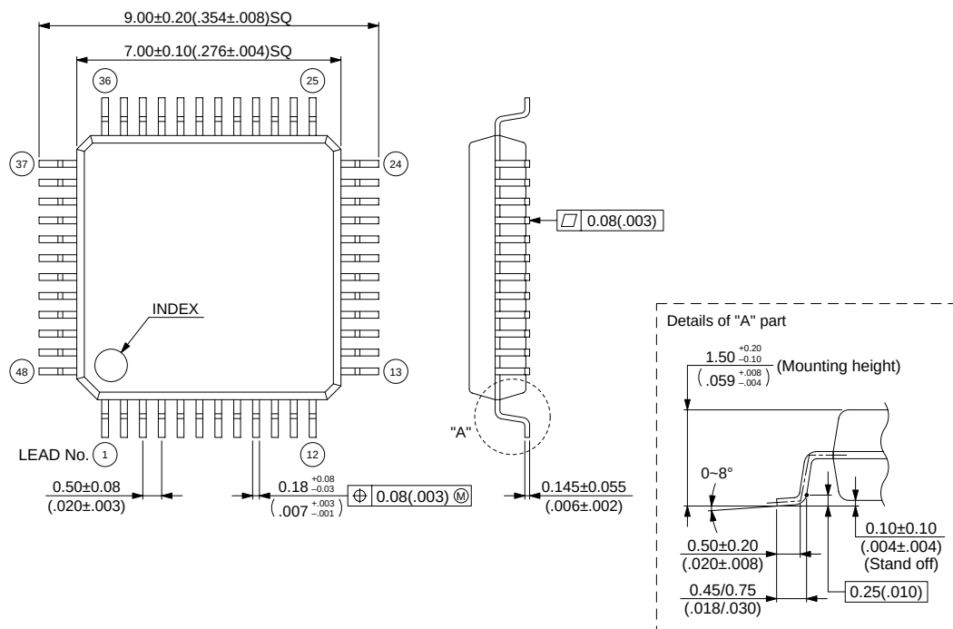
48-pin Plastic LQFP (FPT-48P-M05)
