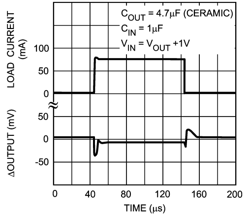
Load Transient
