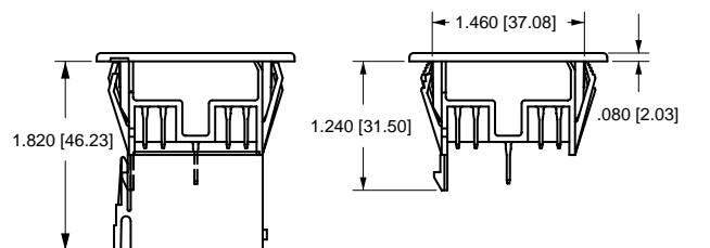
VH2 HOLE PLUG (With wing serrations)
