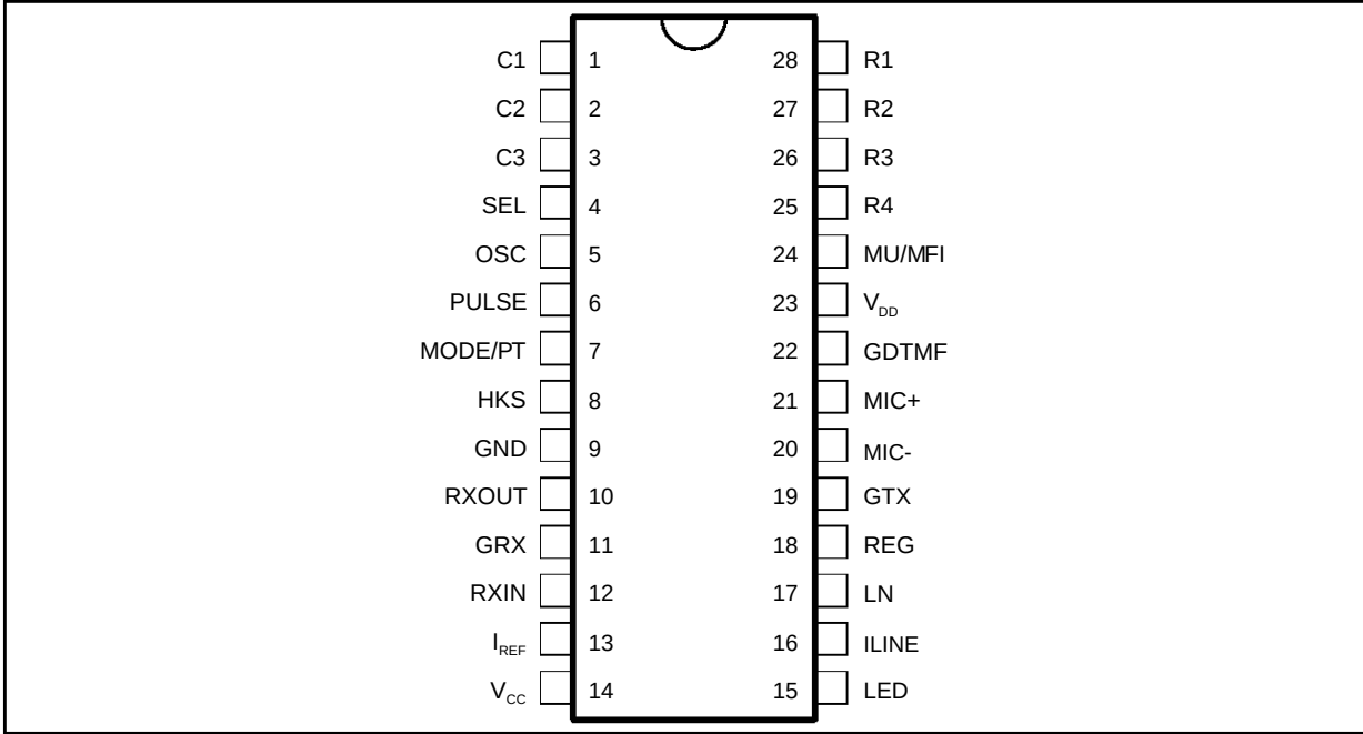
Figure 1 : Keyboard Configuration
