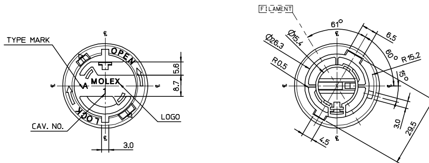
VIEW "A"
