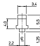
DETAIL "B" SCALE 2:1
